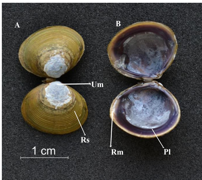
FIGURE 2. Specimens of Corbicula largillierti from Del Valle River in the locality of La Puerta (28°11'13.39" S, 65°46'43.15" W) Umbo (Um) and surface ribs (Rs) are marked in the external view (A). Rostrum area (Rm) and Pallial line (Pl) are indicated on the inner view (B).
