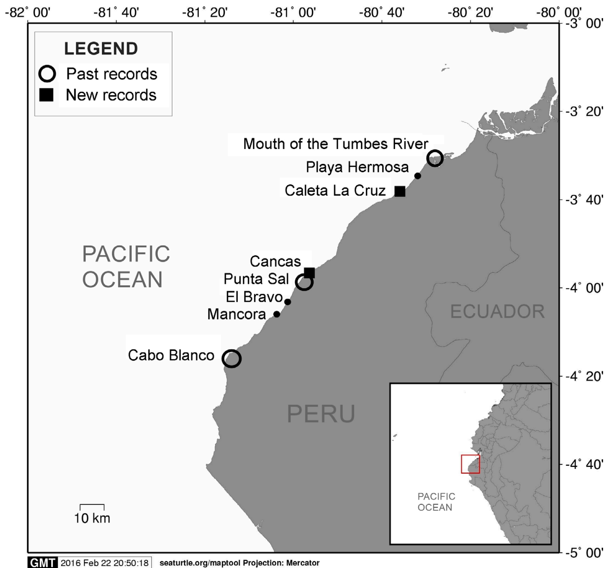
Figure 1. Map showing the locations of Pristis pristis recorded in Peru. Circles are previous reports of landings: mouth of the Tumbes River (Chirichigno and Cornejo 2001), Punta Sal and Cabo Blanco (McDavitt pers. comm. 2016). Squares show new landing reports: Caleta La Cruz (2014) and Cancas (2015), both in the Department of Tumbes. Map created using Maptool (Seaturtle.org 2002).
